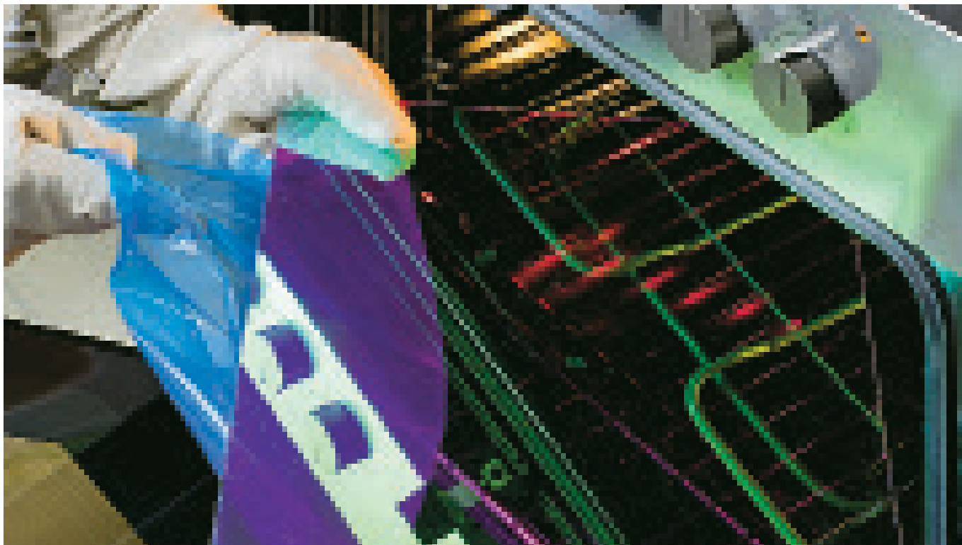
The PLEXIGLAS® sheet is placed in the airflow oven without its protective masking. Wear gloves to remove the sheet from the oven!
